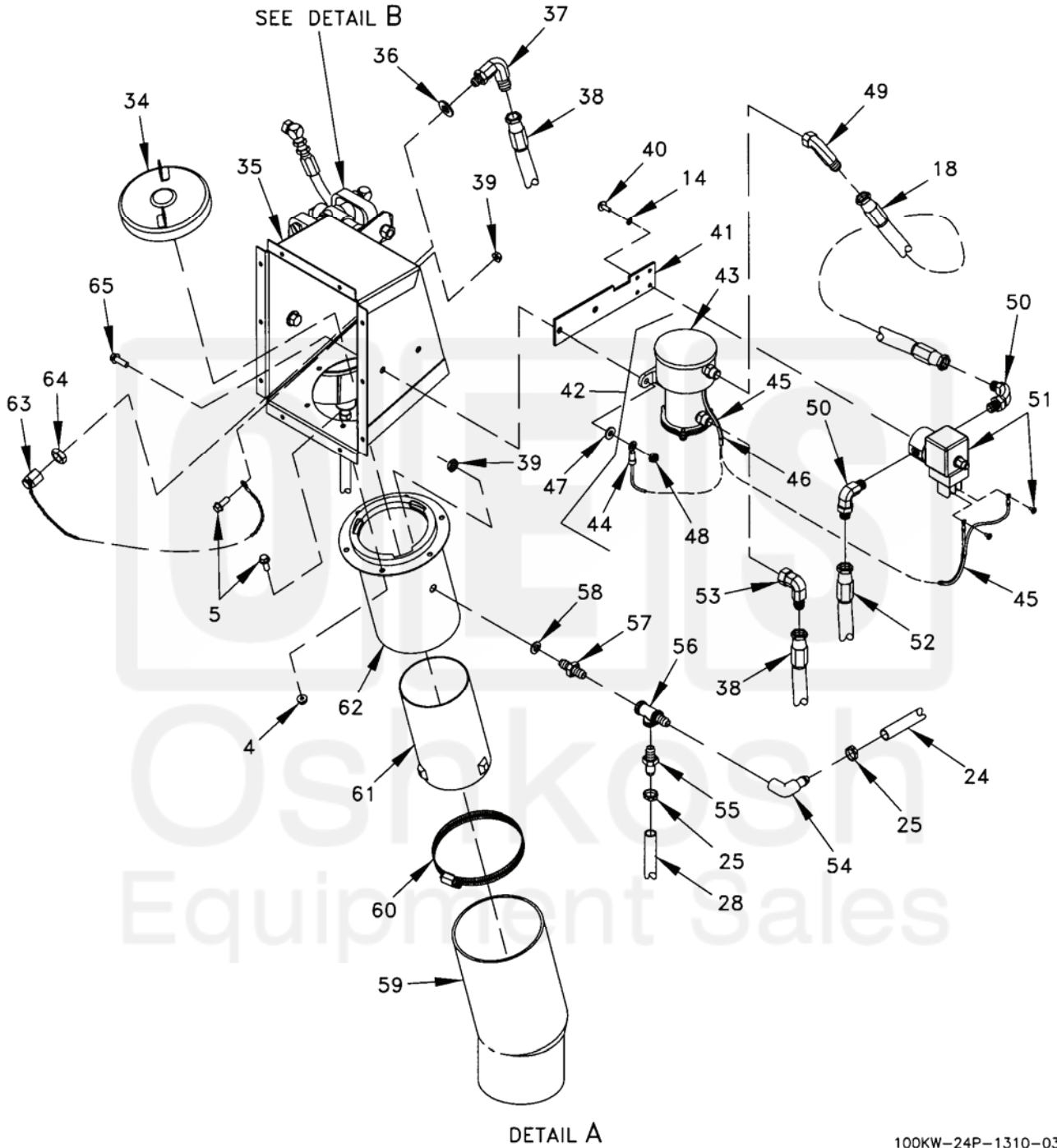
Figure 12. Fuel System Installation (Sheet 3 of 4).
